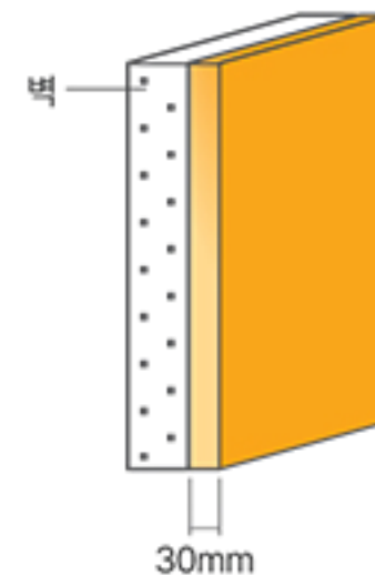
VIP(0.0045W/mk) 적용
